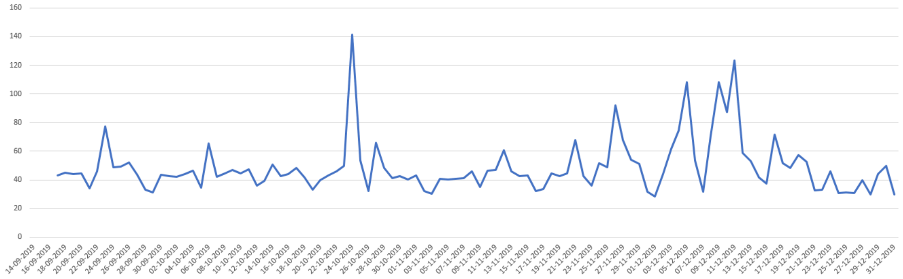
Netbank Classic PIS Average Request Time (in Milliseconds)
