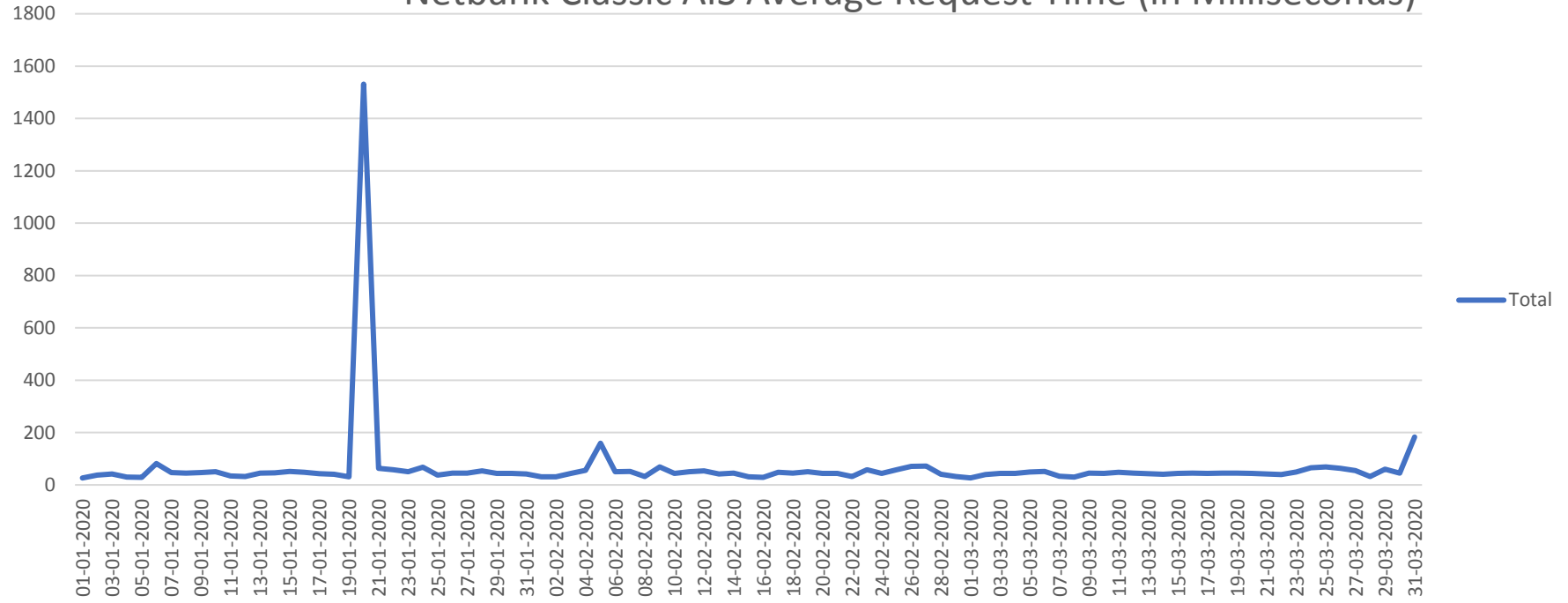
Netbank Classic AIS Average Request Time (in Milliseconds)
